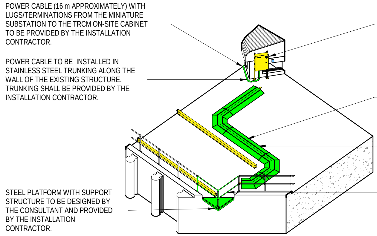
DETAIL B - CABLE PROTECTOR AND PLATFORM NTS
