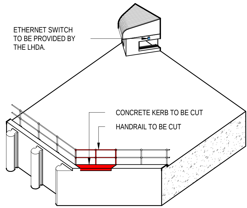
DETAIL B - PRE-MODIFICATION NTS
